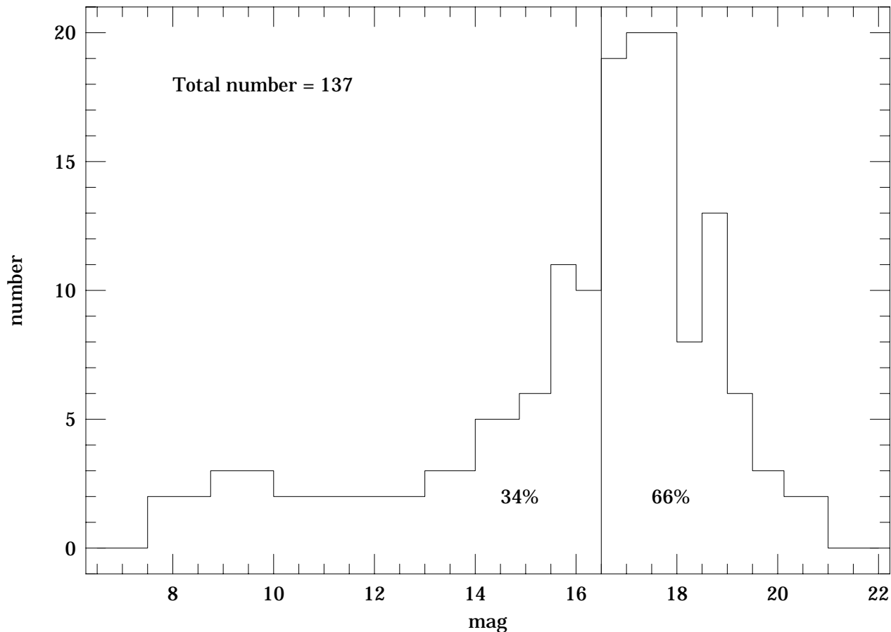
Figure 3: The distribution of the comet brightnesses during the discovery based on the data published in IAU Circulars
