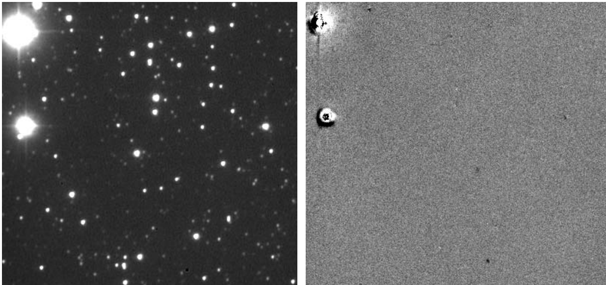
Figure 5: Left panel: Raw image of the field placed in the Galactic planet. Right panel: Image obtained after the subtraction of the reference frame from the raw one
